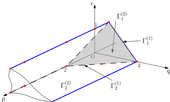
Figure 1 The polyhedron \Gamma for the Hamiltonian function (9) in coordinates p, q, r .
